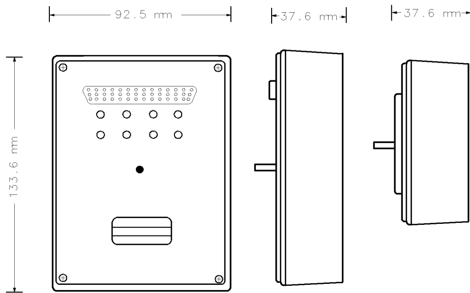
Figure 1-2. 85629B Dimensions
