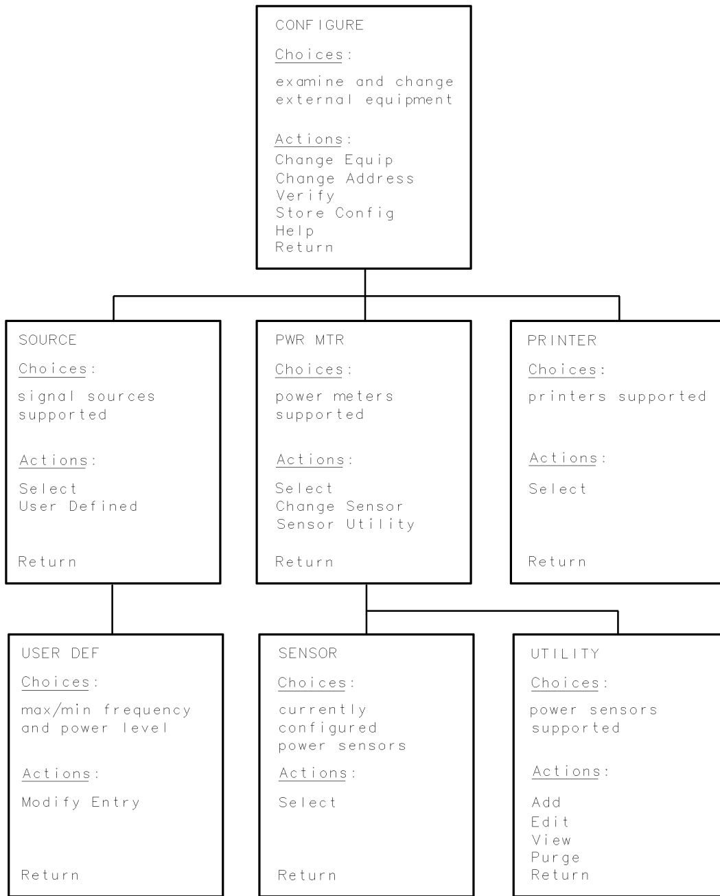
Figure 3-3. System Configuration Menu Structure
